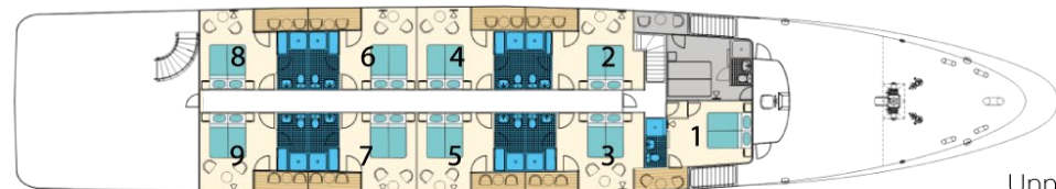
Upper deck
